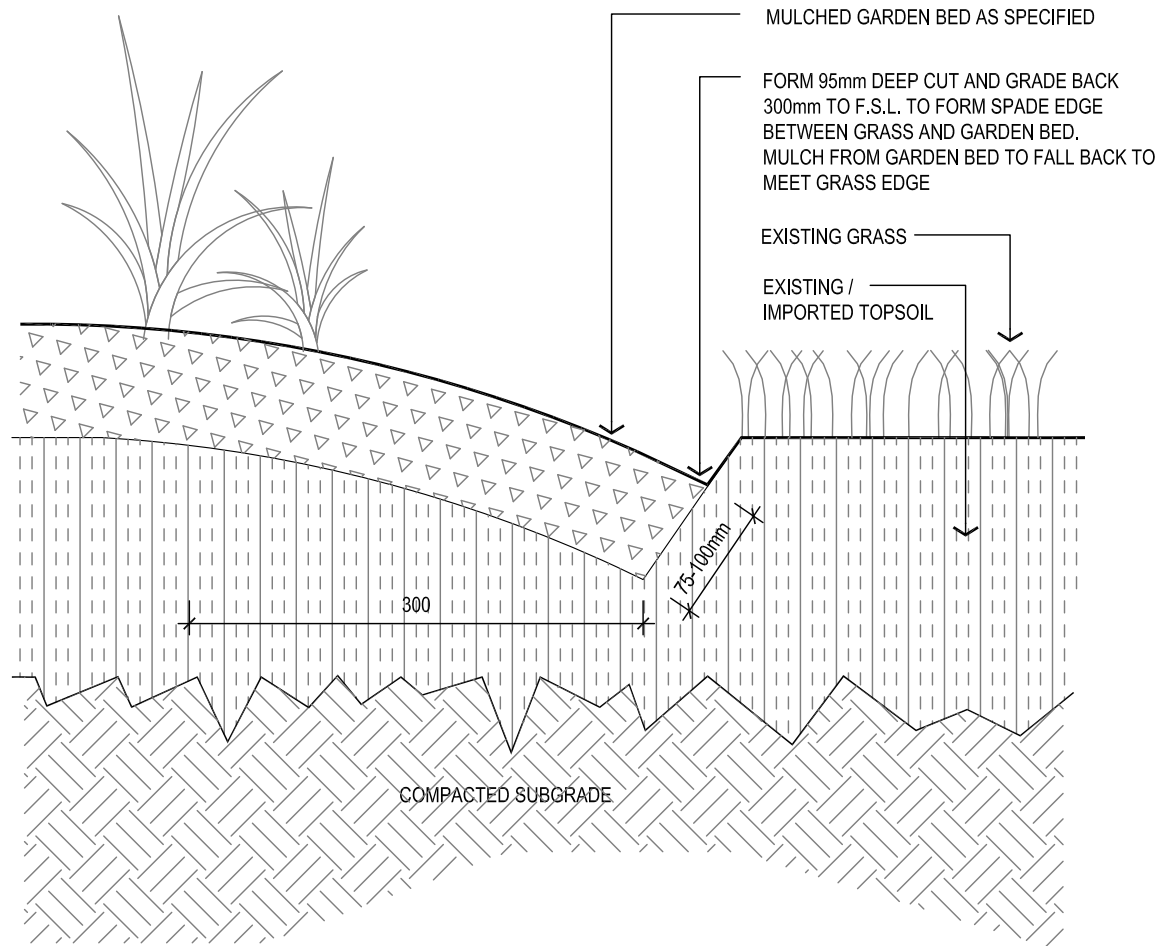
SPADE EDGING DETAIL SECTION
