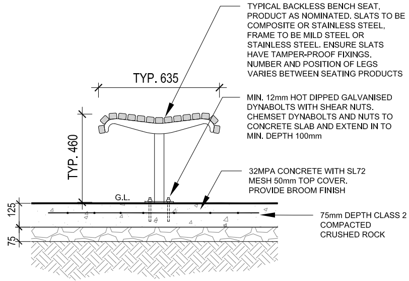
01 BENCH BOLTED DOWN TO CONCRETE SLAB ELEVATION 1:20
