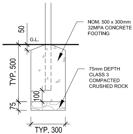
02 EXTENDED LEG FOOTING DETAIL ELEVATION 1:20
