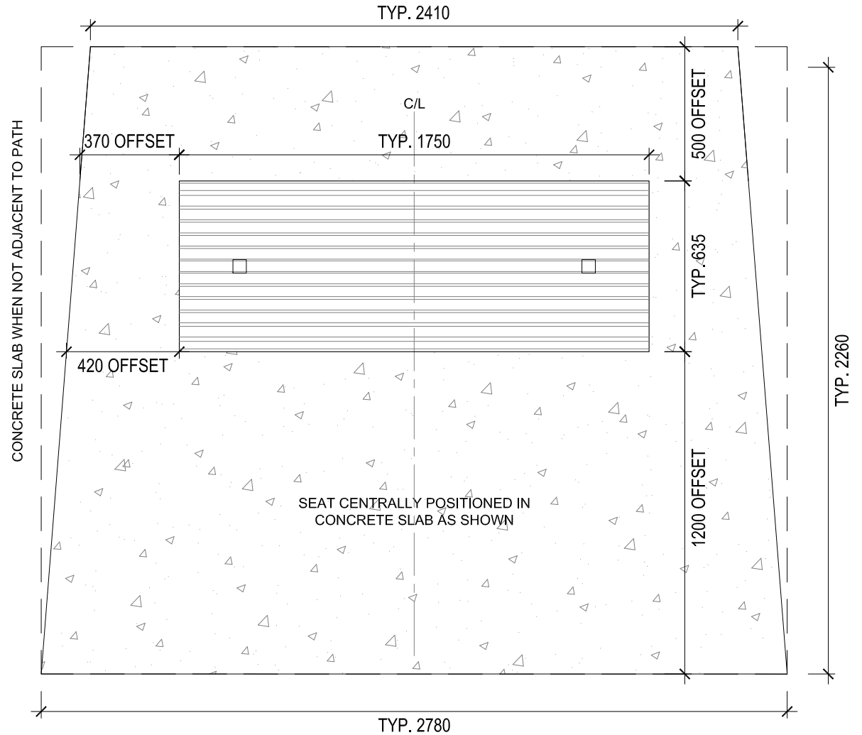
03 SEAT LAYOUT: ADJACENT TO PATH PLAN 1:20
