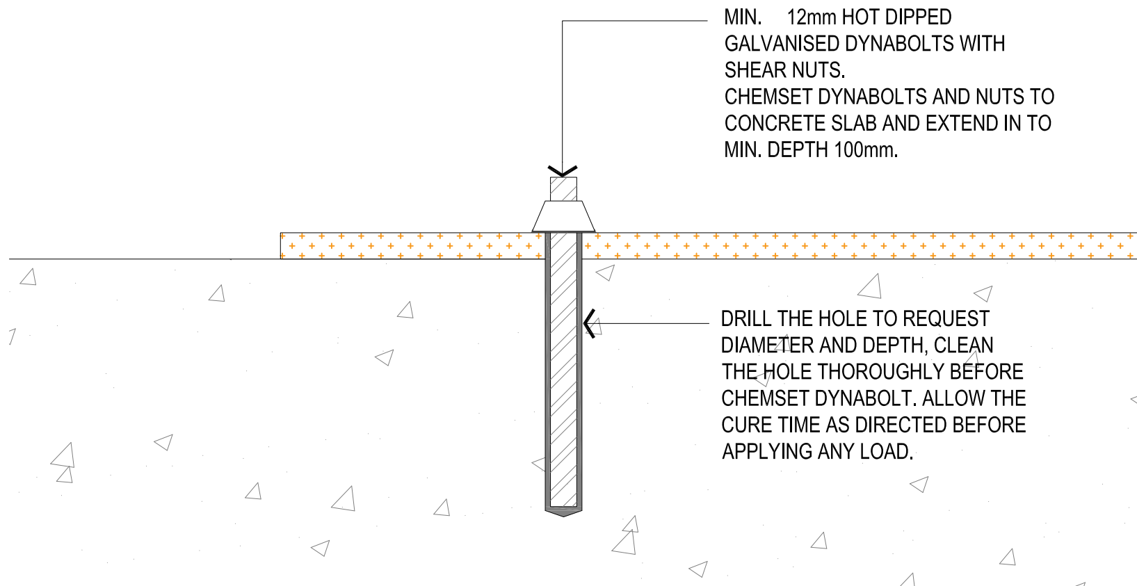
01 FIXING DETAIL SECTION 1:2
