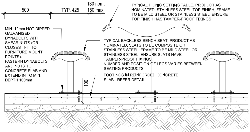
02 PICNIC SETTING - CURVED BENCH SEAT ELEVATION / SECTION
