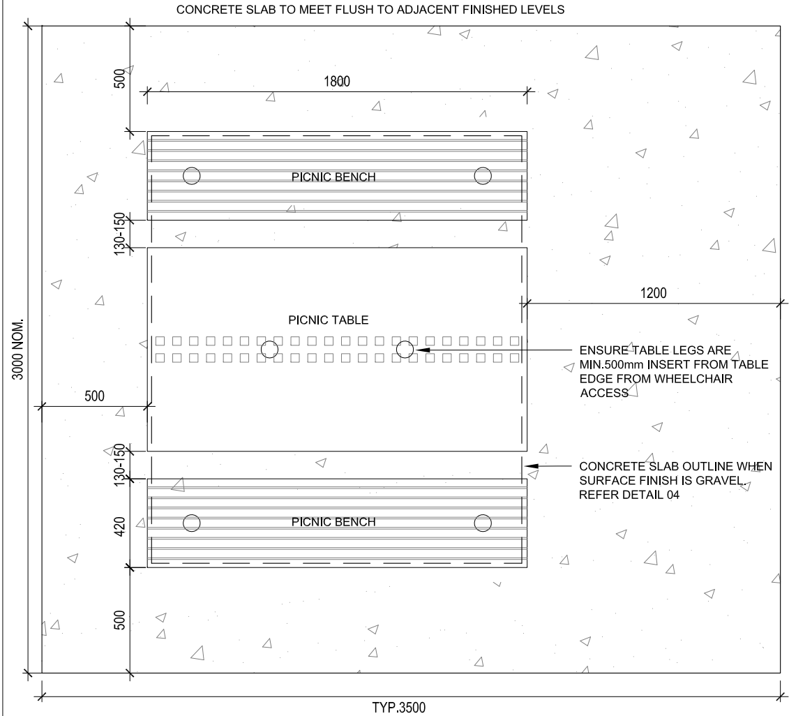
01 TYPE B PICNIC SETTING LAYOUT PLAN
