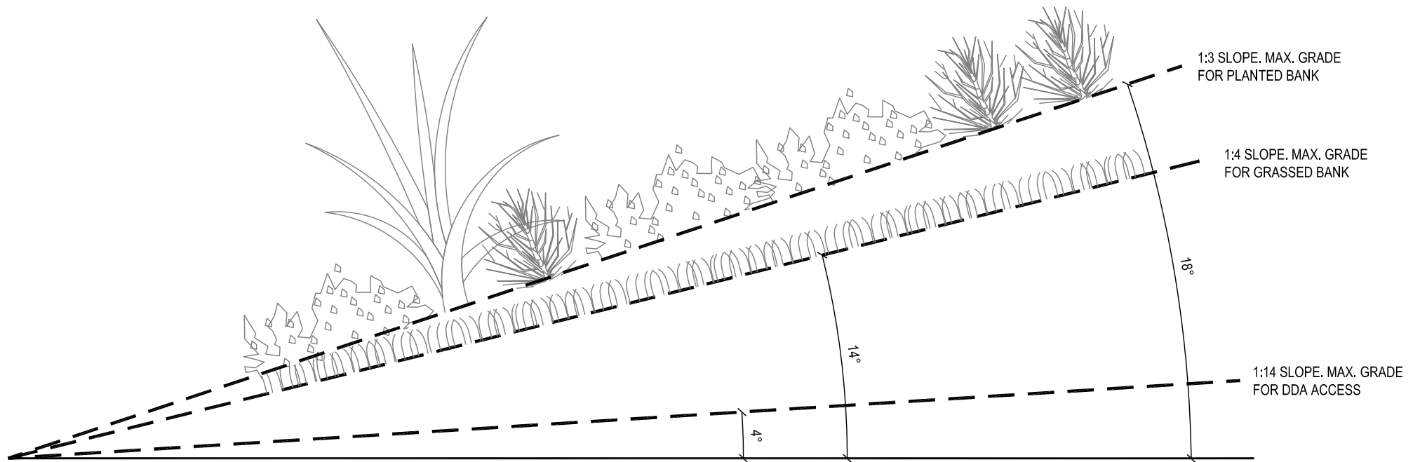
GRADE FOR PLANTING AND ACCESS CROSS SECTION
